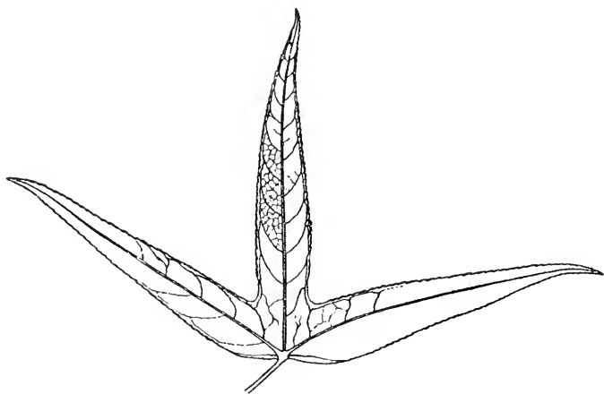
FIGURE 2.—Reconstruction of Liquidambar fontanella . \times \frac{1}{2}
